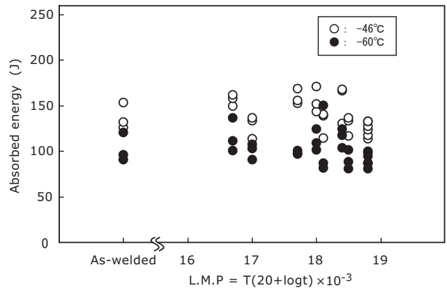
Figure 2: Charpy impact absorbed energies of DW-A55LSR weld metal as a function of SR parameter (L.M.P.: Larson-Miller Parameter).
