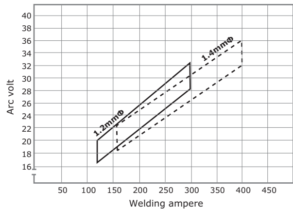
Figure 4: Proper range of welding amperage and arc voltage with DW-55L (1.2 and 1.4 mmØ).
