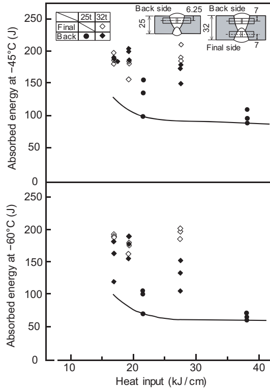
Figure 1: Impact absorbed energies of LB-62L (4 mmØ) weld metals as a function of heat input in welding double-V groove joints in flat, horizontal and vertical-up positions (As-weld; Power source: AC).
