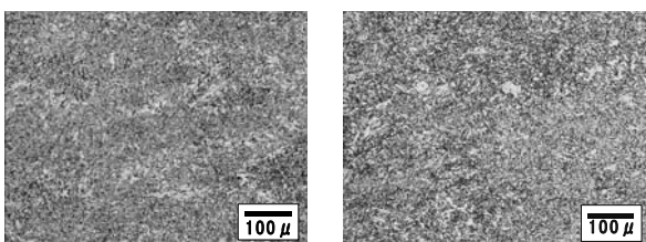
Figure 1: Ti-B micro-alloyed fine microstructures of DW-62L (left) and DW-A62L (right) weld metals.
