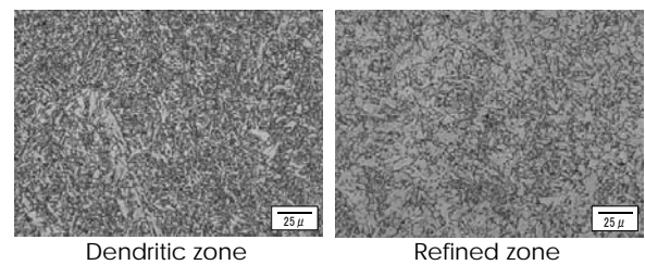
Figure 1: Fine microstructures of DW-A81Ni1 as-welded weld metal on the final side in the vertical position.
