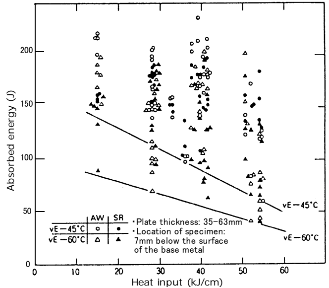
Figure 1: Charpy impact absorbed energy of LB-52NS weld metals as a function of heat input in welding thick-section butt joints.
