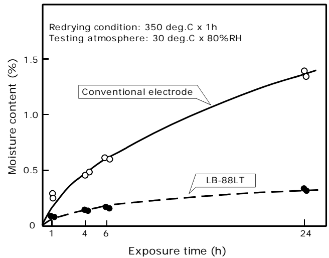
Figure 2: A comparison between LB-88LT and conventional electrode on moisture pick up in the testing atmosphere.
