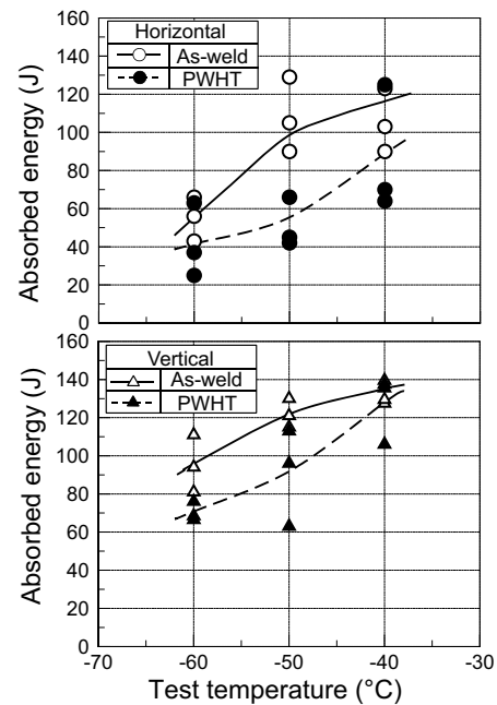
Figure 2: Absorbed energies in Charpy impact testing of DW-A81Ni1 weld metal in the as-welded and PWHT (580°C x 2h) conditions (Base metal: 50-mm thick FH36; Groove: double-bevel; Specimen location: final side).
