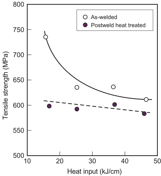
Figure 2: Tensile strength of NB-1SJ weld metal as a function of Heat input in the as-welded and postweld heat treated (600 °C x 2h) conditions.
