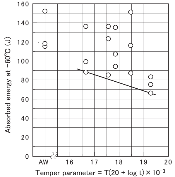
Figure 2: Charpy impact test results of LB-65L weld metal in the as-welded and postweld heat treated conditions (PWHT/temper parameter: 560°C x 1h/16.66; 580°C x 4h/17.57; 620°C x 1h/17.86; 620°C x 5h/18.48; 620°C x 40h/19.29).
