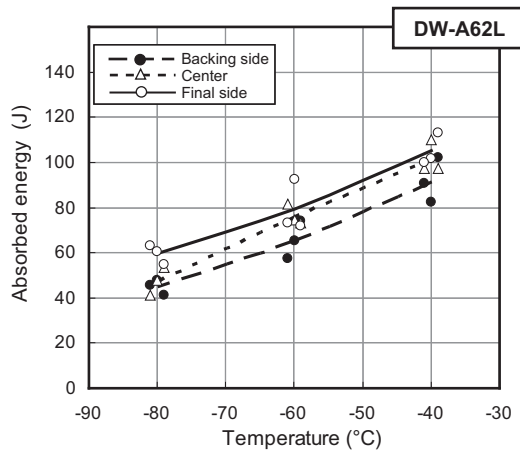
Figure 2: Charpy impact absorbed energies of weld metals tested with 60-mm thick double-V groove joints and 1.2 mmØ wires in vertical welding.
