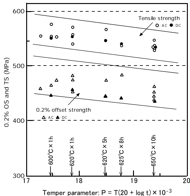
Figure 3: Effect of PWHT conditions on tensile properties of LB-52NS deposited metal.
