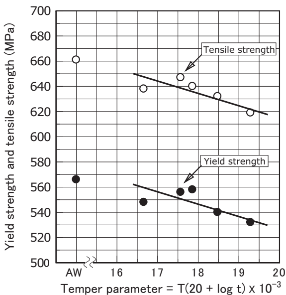
Figure 1: Tension test results of LB-65L weld metal in the as-welded and postweld heat treated conditions (PWHT/temper parameter: 560°C x 1h/16.66; 580°C x 4h/17.57; 620°C x 1h/17.86; 620°C x 5h/18.48; 620°C x 40h/19.29).
