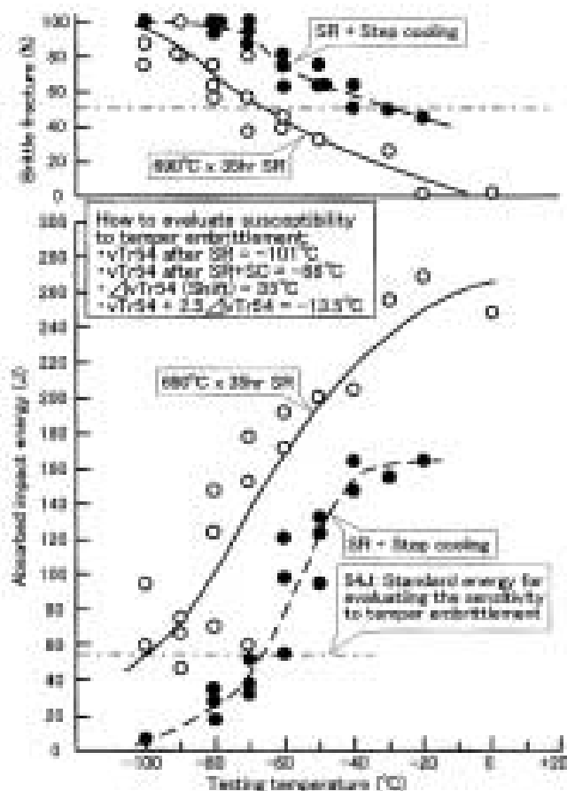
Fig. 1. Temper embrittlement test results of TGS-2CM deposited metal by Charpy impact test
