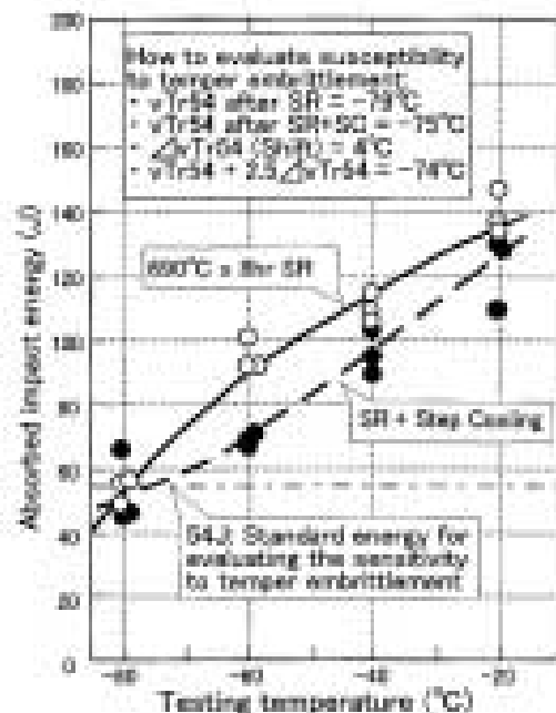
Fig. 3. Temper embrittlement test results of CMA-106N (5 mm) weld metal by Charpy impact test (AC current, flat welding position)
