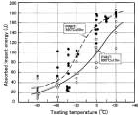
Fig. 2. Charpy impact test results of CMA-106 (5.0 ) deposited metal by AC welding in flat position
