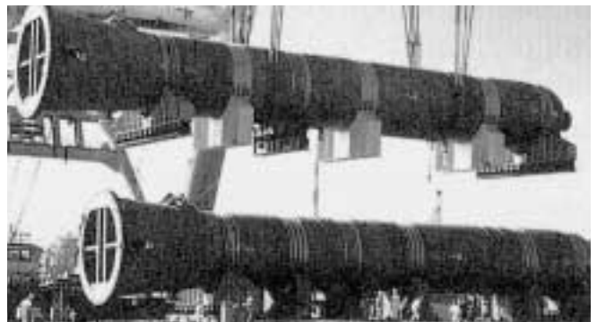
Photo 2. The world's largest heavy oil desulfurization reactor vessel having a shell of 330-mm thick and weighing 1400 tons (Photo source: Welding Technique , Vol.47, Japan Welding Engineering Society)
