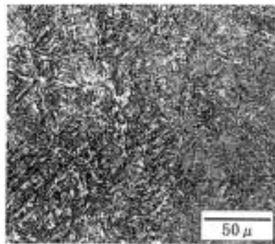
Photo 3. Microstructure of CMA-106H weld metal of fine bainite (2% nital etching)
