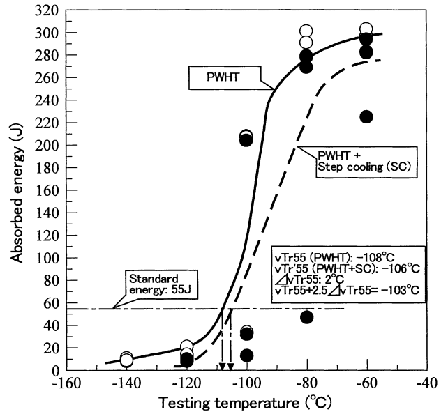
Fig. 5. Charpy impact test results of TGS-2CMH weld metal after PWHT (705 x 7h) and PWHT + Step Cooling (Power source: DCEN; Welding position: flat; Ar shielding)
