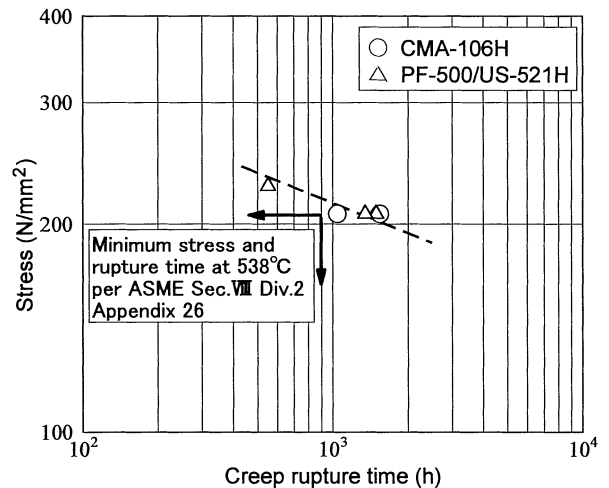
Fig. 6. Creep rupture test results of CMA-106H and PF-500/US-521H weld metals after PWHT (705 x 26h) (Power source: AC; Testing temperature: 538 )
