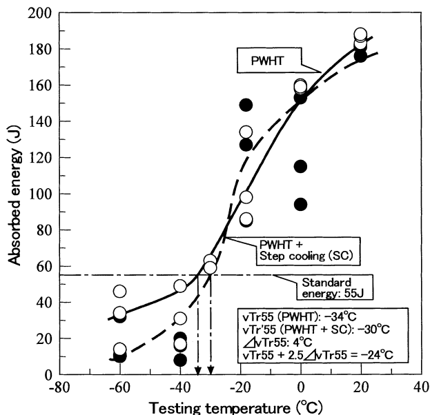
Fig. 4. Charpy impact test results of PF-500/US-521H weld metal after PWHT (705 x 7h) and PWHT + Step Cooling (Power source: AC; Tandem SAW)
