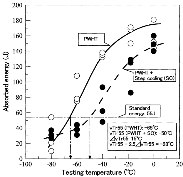
Fig. 3. Charpy impact test results of CMA-106H (4.0 ) weld metal after PWHT (715 x 7h) and PWHT + Step Cooling (Power source: AC; Welding position: flat)
