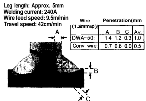
Fig. 3-Penetration test results of DWA-50 in horizontal fillet welding with 80%Ar+20%CO 2 gas shielding
