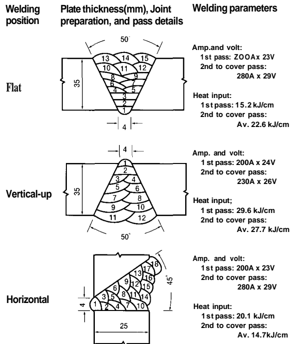
Fig. 4-DWA-50 contributes to highly efficient welding in the shipbuilding industry
