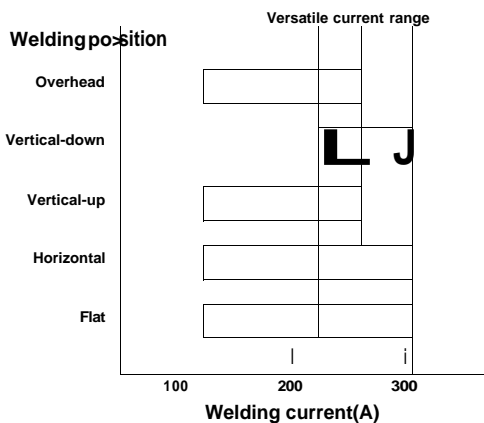
Fig.1- Proper welding current ranges and a versatile current range for all-position welding (DWA-50, 1.2 mm<j>)
